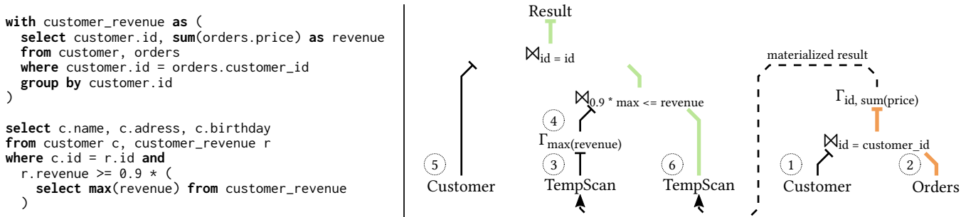
Figure 2: Exemplary SQL OLAP query (left) and corresponding query plan (right) with pipelines. Pipelines continuing through an n -ary operator are marked bold and color-coded. Circled pipeline IDs also denote execution order.
